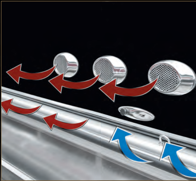
You won't have to deal with mildew or fungus with Avalon's exclusive Flo Thru Ventilation™ Seating. Unlike plastic seating, our exclusive aluminum seat frames have external and internal air flow that dries out the seat compartments while moving and even when the boat is stored!
