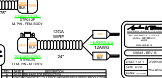
129343 - LONG SUBWOOFER HRNS 2 PIECE HARNESS
